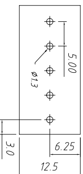
PCB LAYOUT
